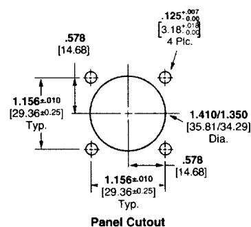
Panel Cutout
