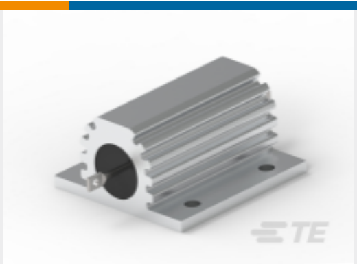
TE Part #4-1625995-0 HSC75 3K0 5%
