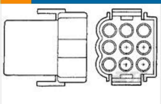
TE Part #1-480673-0 09P .140 MNL CAP PM NAT
