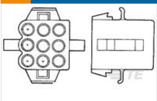
TE Part #1-480672-0 09P .140 MNL PLUG PM NAT
