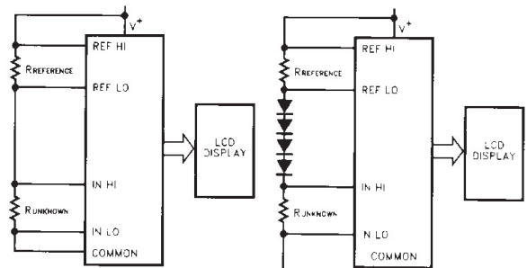
ICL7106 system setup for 2V reference
