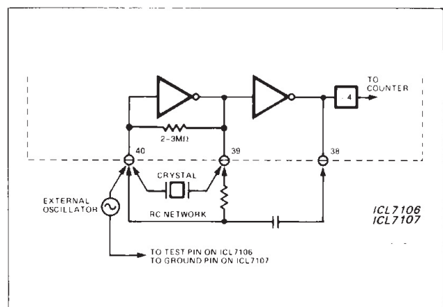
Figure 7. Clock Circuits
