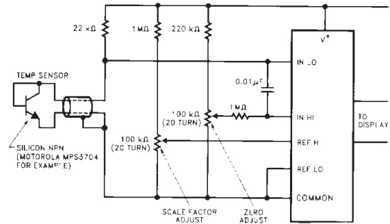
Figure 20. Digital Thermometer
