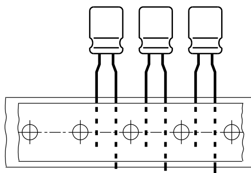
Fig. 3 - Form TFA: Taped in box (ammopack), formed leads, pitch F = 5 mm
