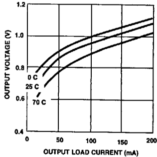
Output Voltage vs Load Current (NE590)
