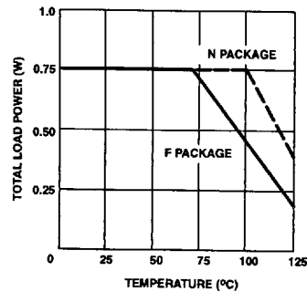
Total Load Power vs Temperature (NE591)
