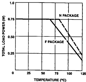
Total Load Power vs Temperature (NE590)
