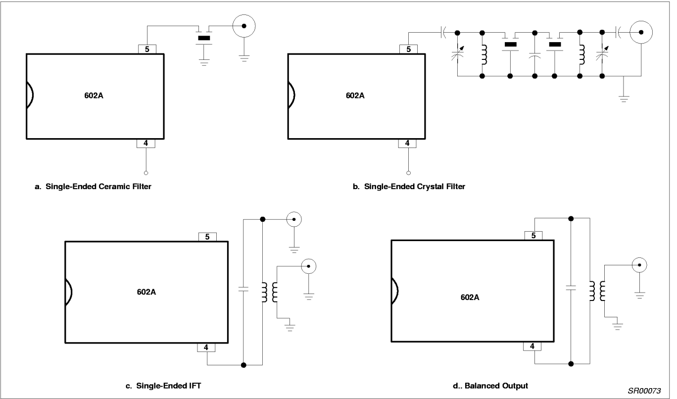
Figure 6. Output Configuration
