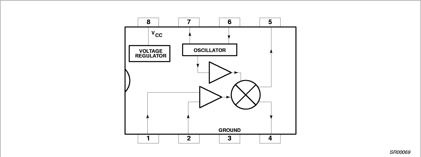
Figure 2. Block Diagram
