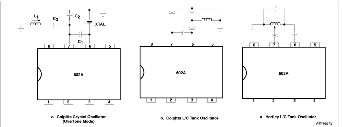
Figure 7. Oscillator Circuits
