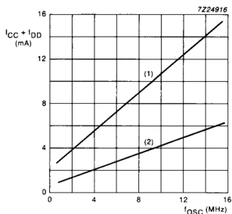
Fig.13 Typical values of maximum supply current ( I_{CC} + I_{DD} ) as a function of the oscillator frequency ( f_{osc} ) at V_{CC(max.)} = 5.5\text{ V} ; T_{amb} = 0\text{ to }+70\text{ }^{\circ}\text{C} .
