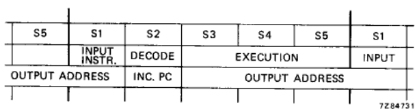
Fig. 11 Instruction cycle.
