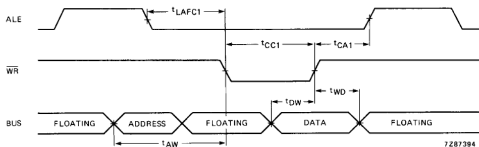
Fig.15 Write to external data memory.
