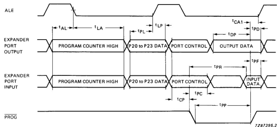
Fig.17 Port 2 timing.
