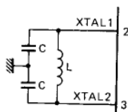
Fig. 7 LC oscillator mode.
