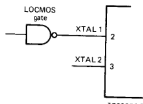
Fig. 6 Driving from an external source.
