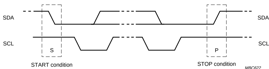
Fig.5 Definition of start and stop conditions.
