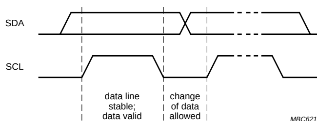
Fig.4 Bit transfer.
