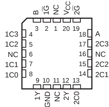
SN54HC153 . . . FK PACKAGE (TOP VIEW)
