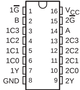
SN54HC153 . . . J OR W PACKAGE SN74HC153 . . . D, N, NS, OR PW PACKAGE (TOP VIEW)
