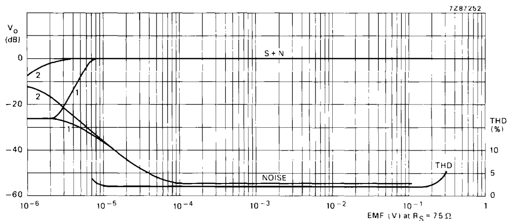
Fig. 3 A.F. output voltage ( V_o ) and total harmonic distortion (THD) as a function of the e.m.f. input voltage (EMF) with a source impedance ( R_S ) of 75\ \Omega : (1) muting system enabled; (2) muting system disabled.
