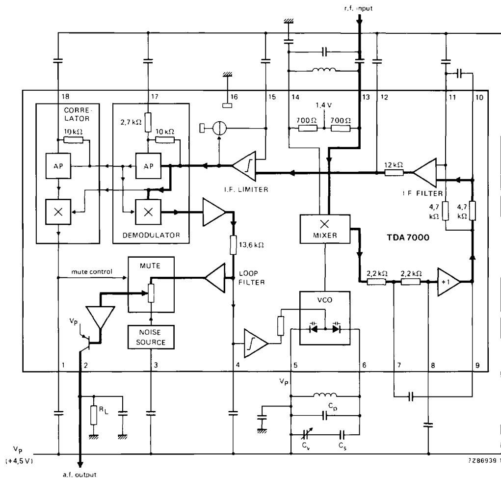
Fig. 1 Block diagram.
