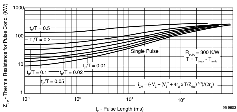
Figure 11. Thermal Response
