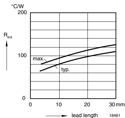
Figure 4. Thermal Resistance vs. Lead Length
