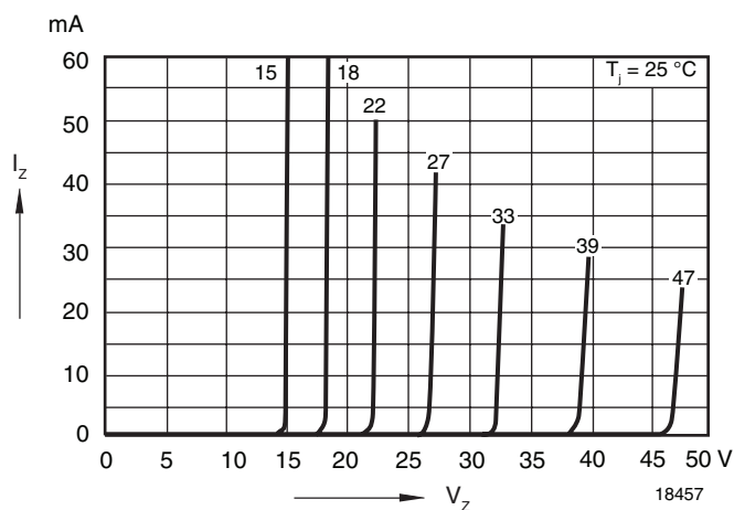
Figure 8. Breakdown Characteristics
